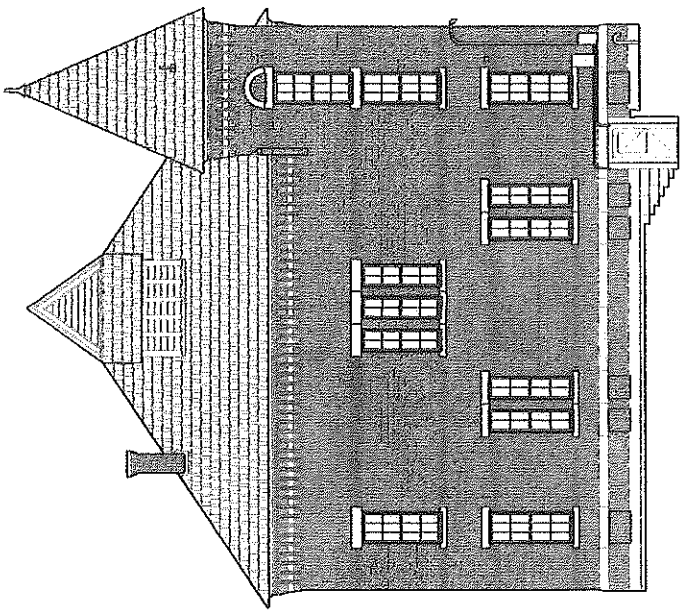
1 SOUTH ELEVATION - PROPOSED SCALE: 1/8" = 1'-0"
