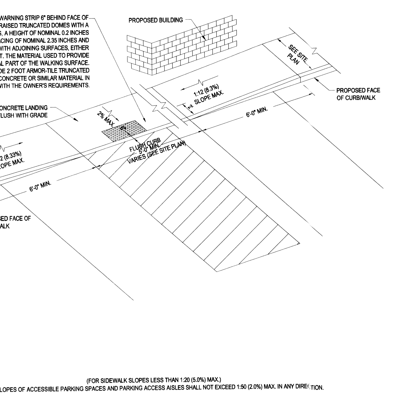
SLOPED WALK DETAIL
