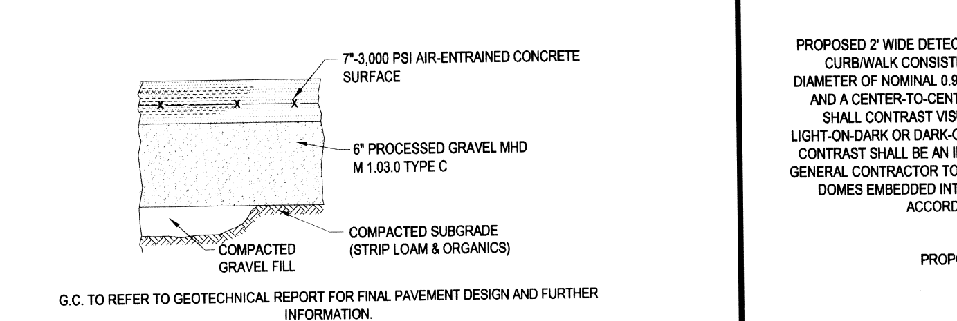
CONCRETE MAT SECTION
