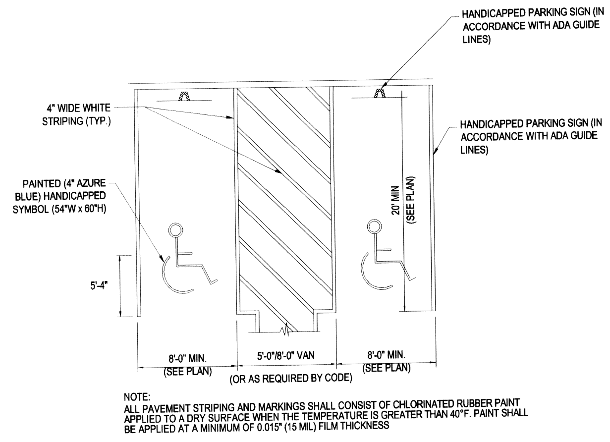
HANDICAPPED STALL MARKINGS & PARKING LOT STRIPING DETAIL
