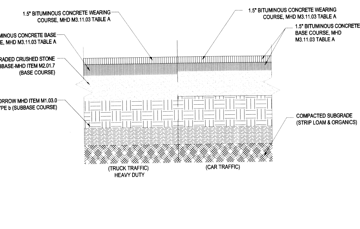
PAVEMENT SECTION
