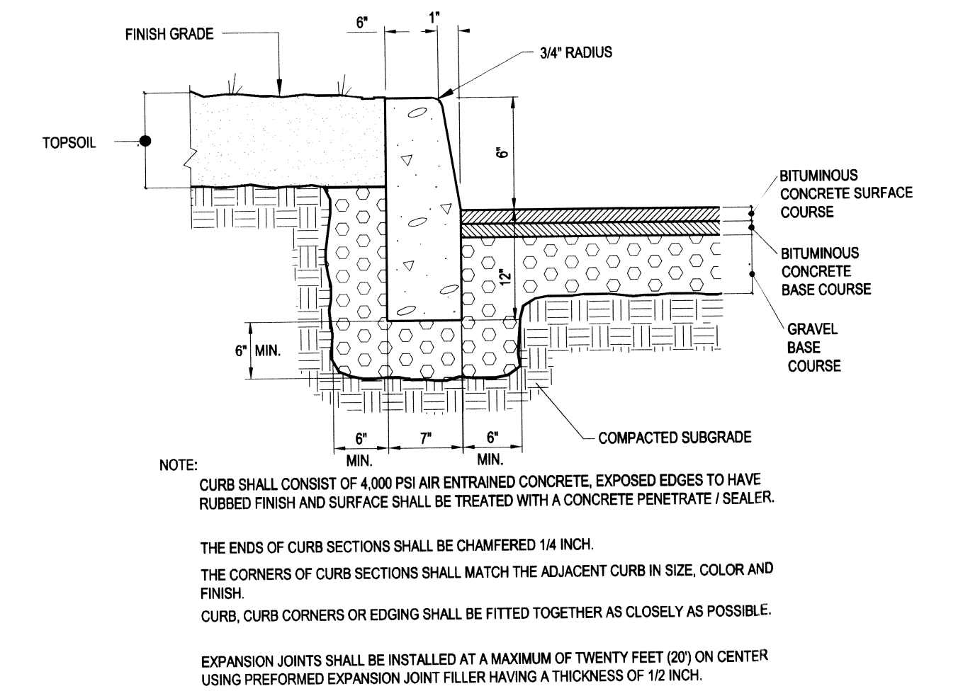
PRECAST CONCRETE CURB DETAIL
