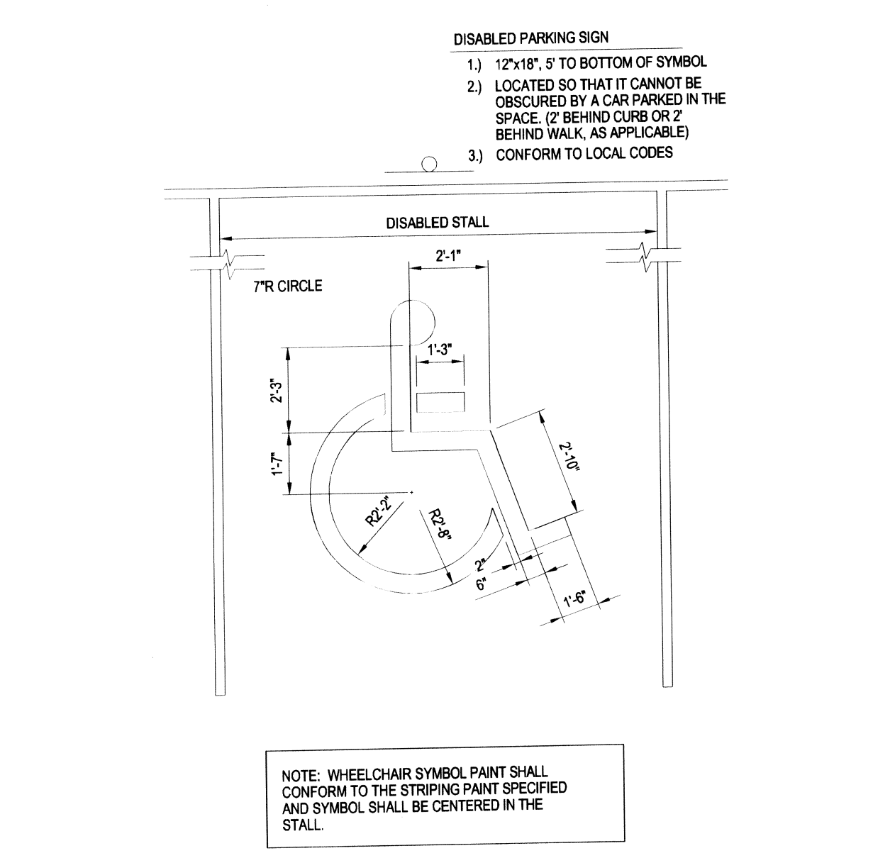
DISABLED SPACE PARKING PAINTING DETAIL
