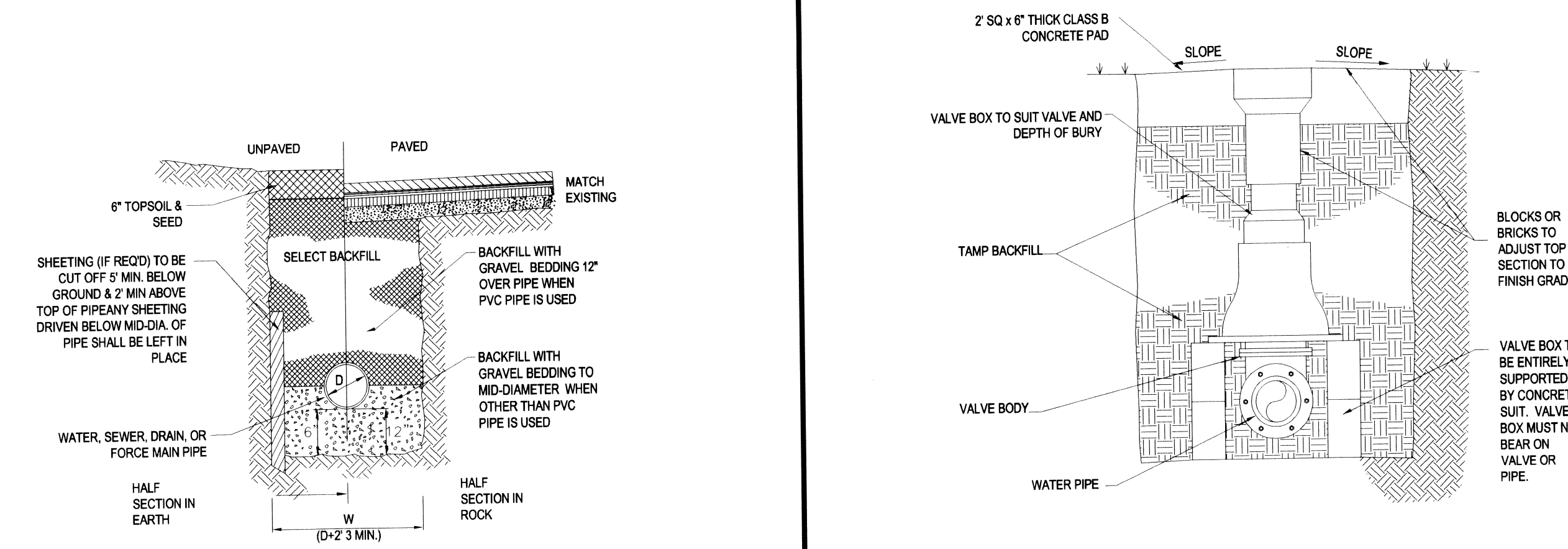
GATE VALVE
