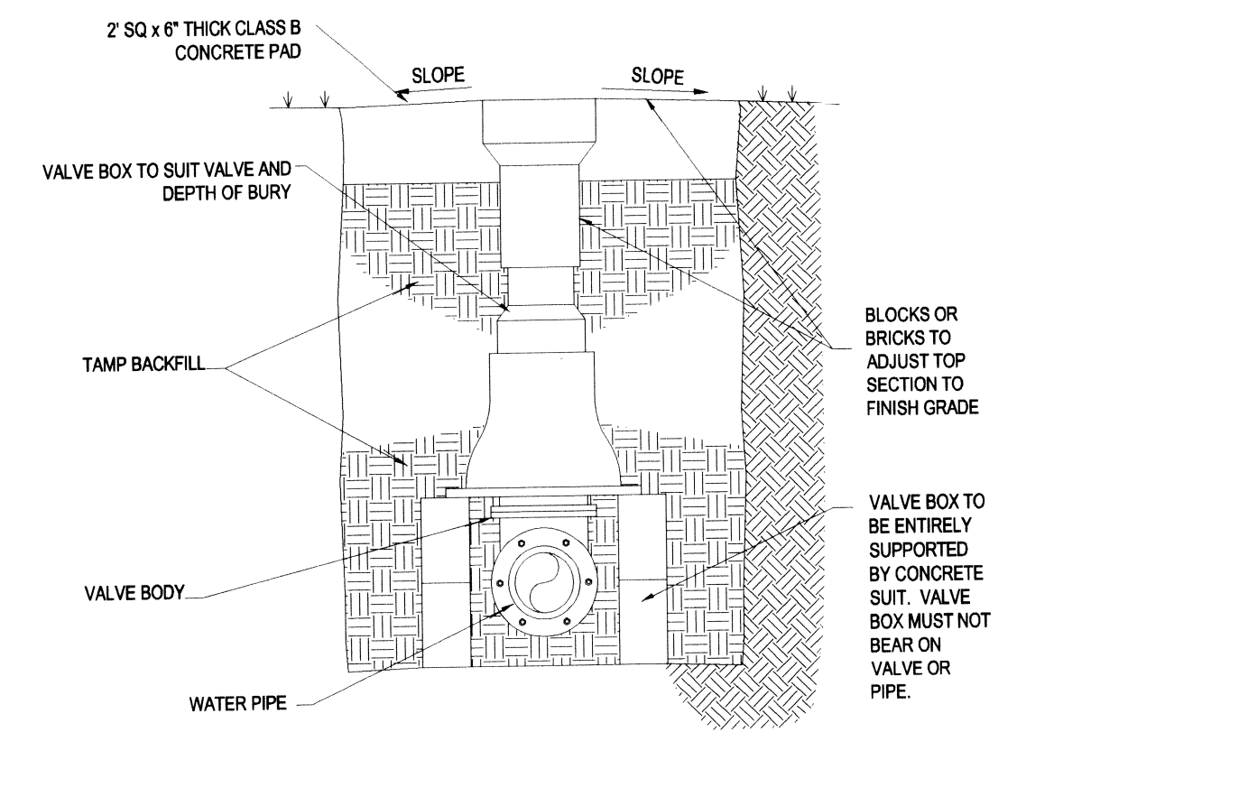
GATE VALVE
