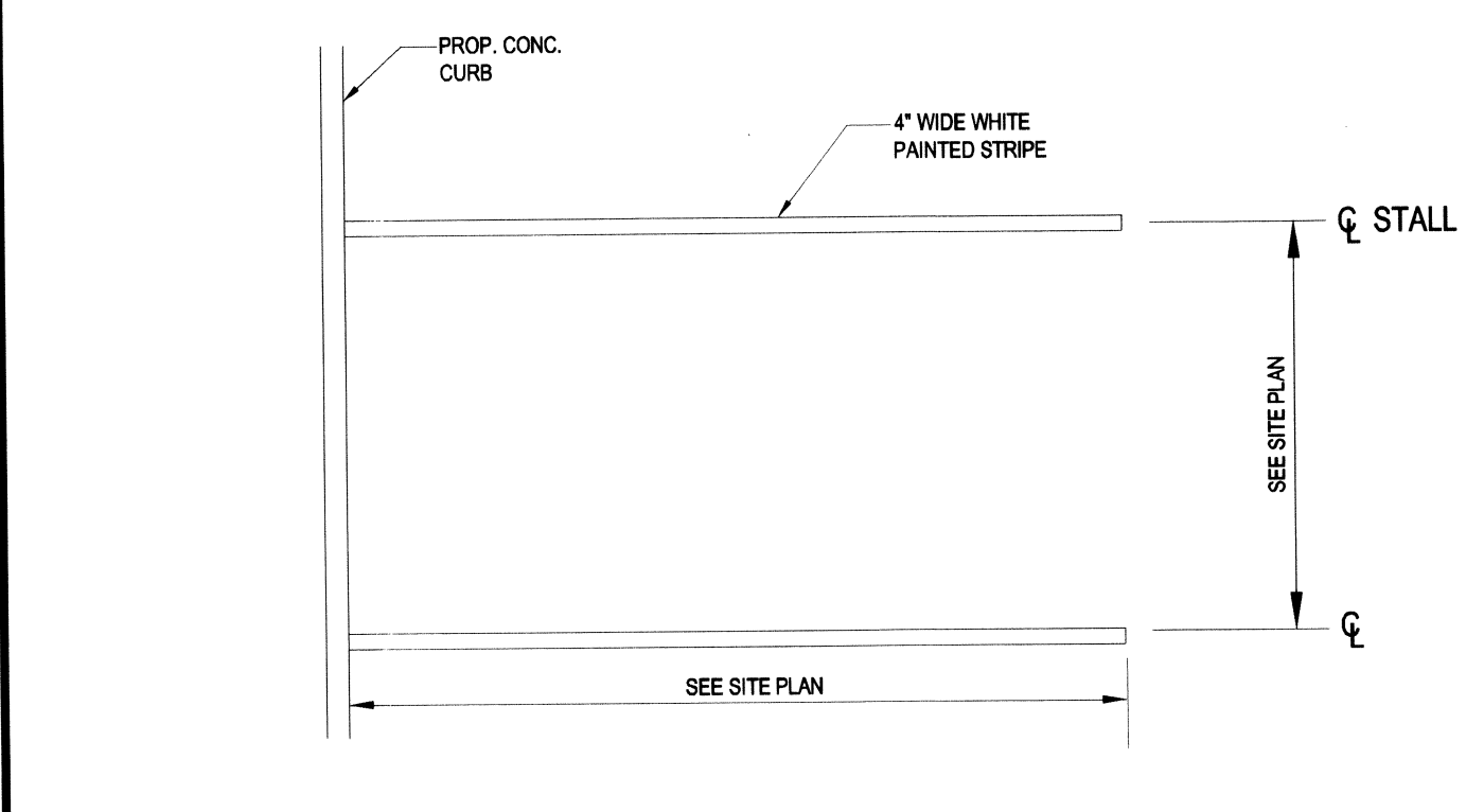
PROPOSED PARKING STALL MARKINGS
