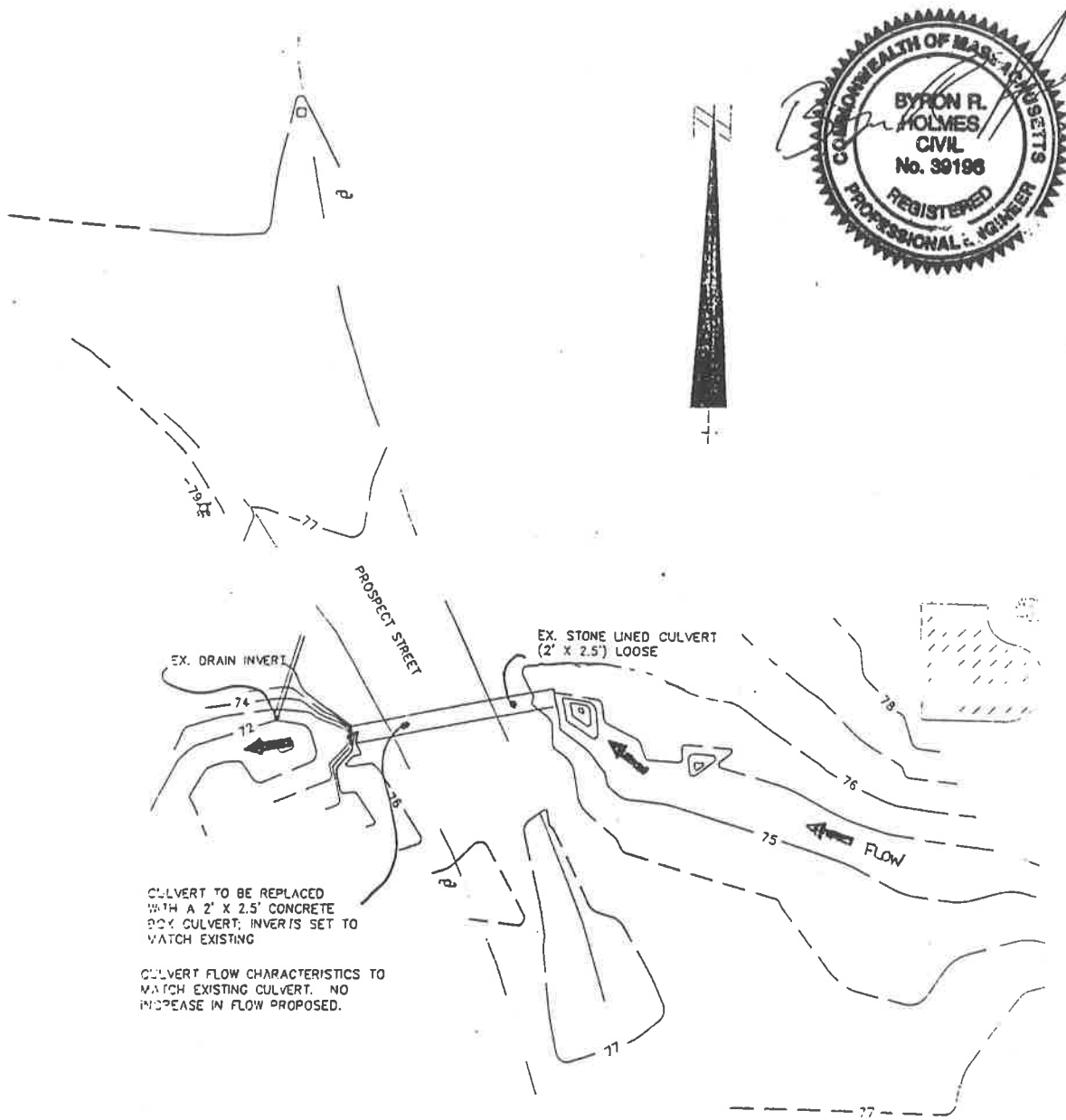
PROSPECT STREET CULVERT Scale 1 inch = 40 feet
