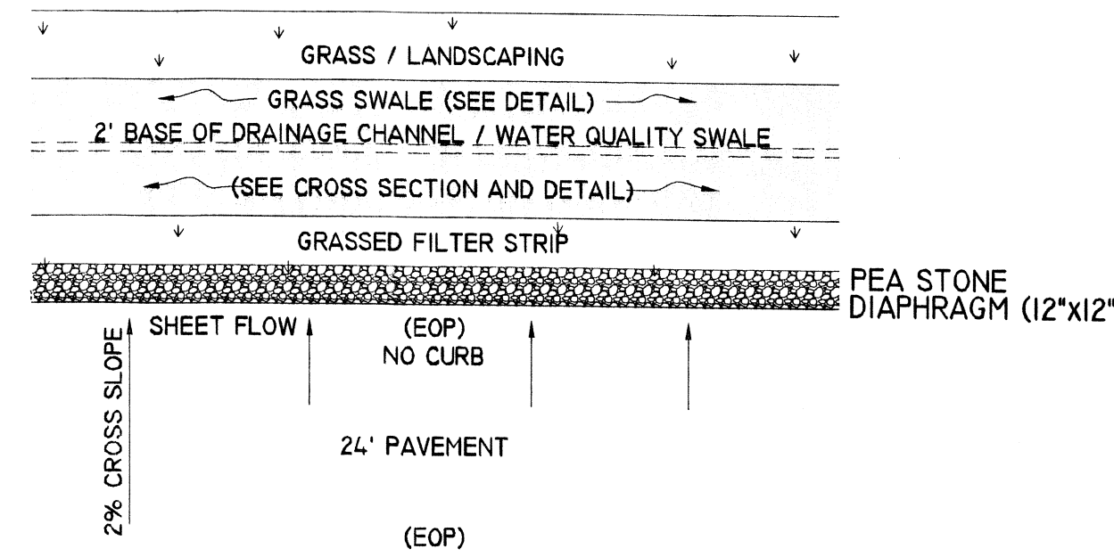
PEA STONE DIAPHRAGM DETAIL
