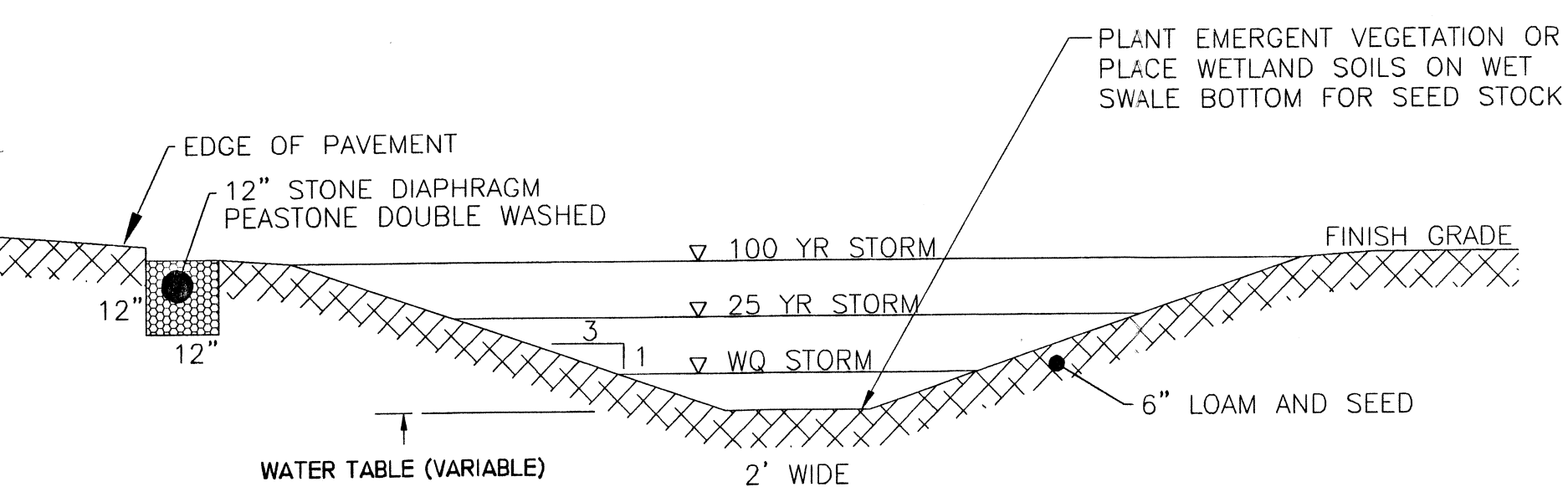
WATER QUALITY SWALE
