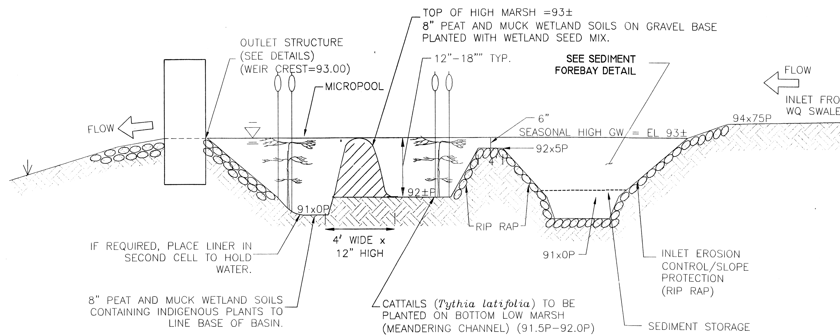
CONSTRUCTED (POCKET) WETLAND SECTION
