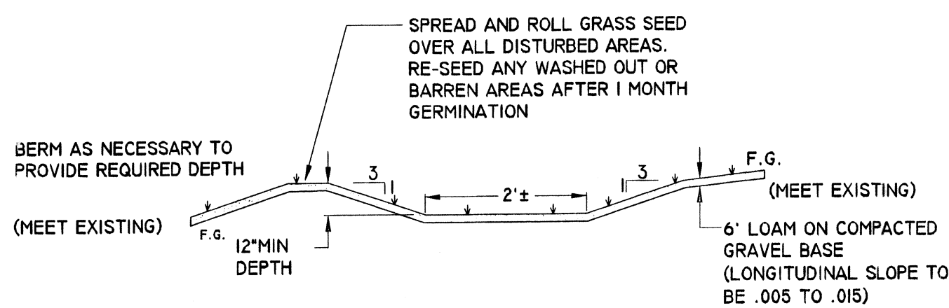
DRAINAGE CHANNEL - SECTION
