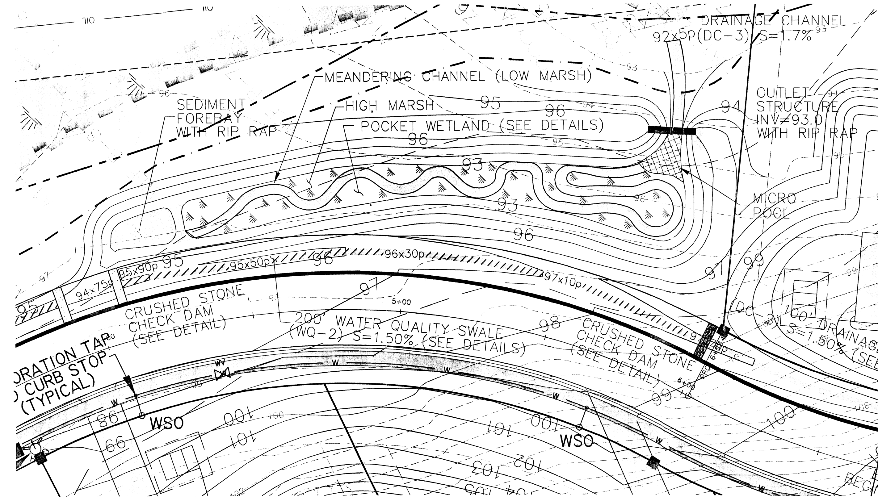
CONSTRUCTED (POCKET) WETLAND DETAIL
