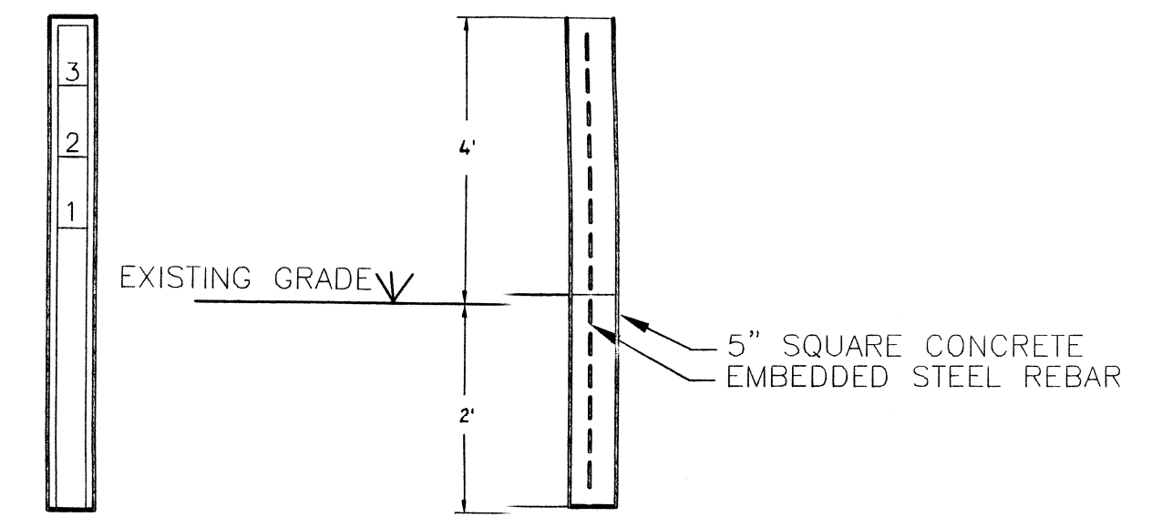
CONCRETE SEDIMENT MARKER
