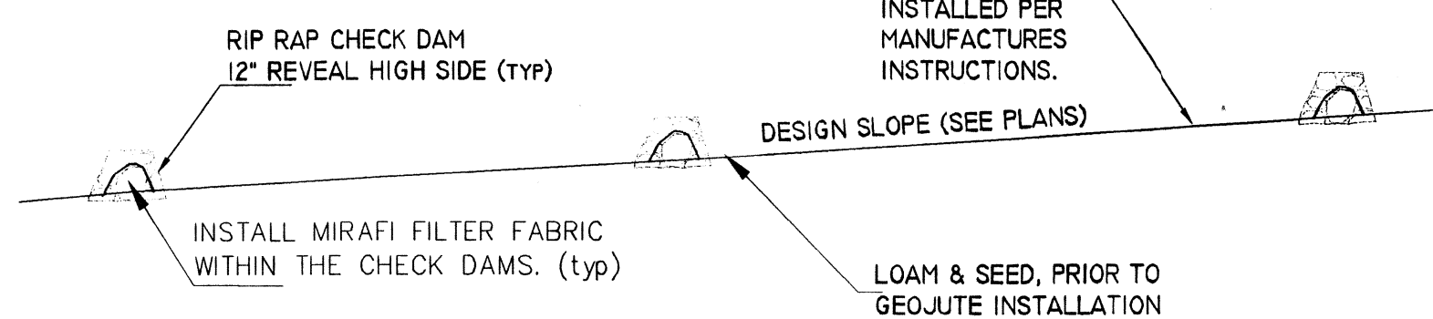
WATER QUALITY SWALE - PROFILE
