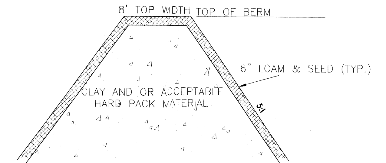
TYPICAL DIKE SECTION DETAIL
