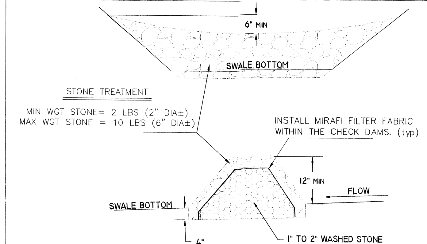
CHECK DAM DETAIL
