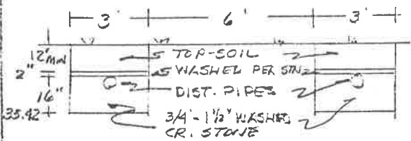
LEACHING TRENCHES TYPICAL SECTION
