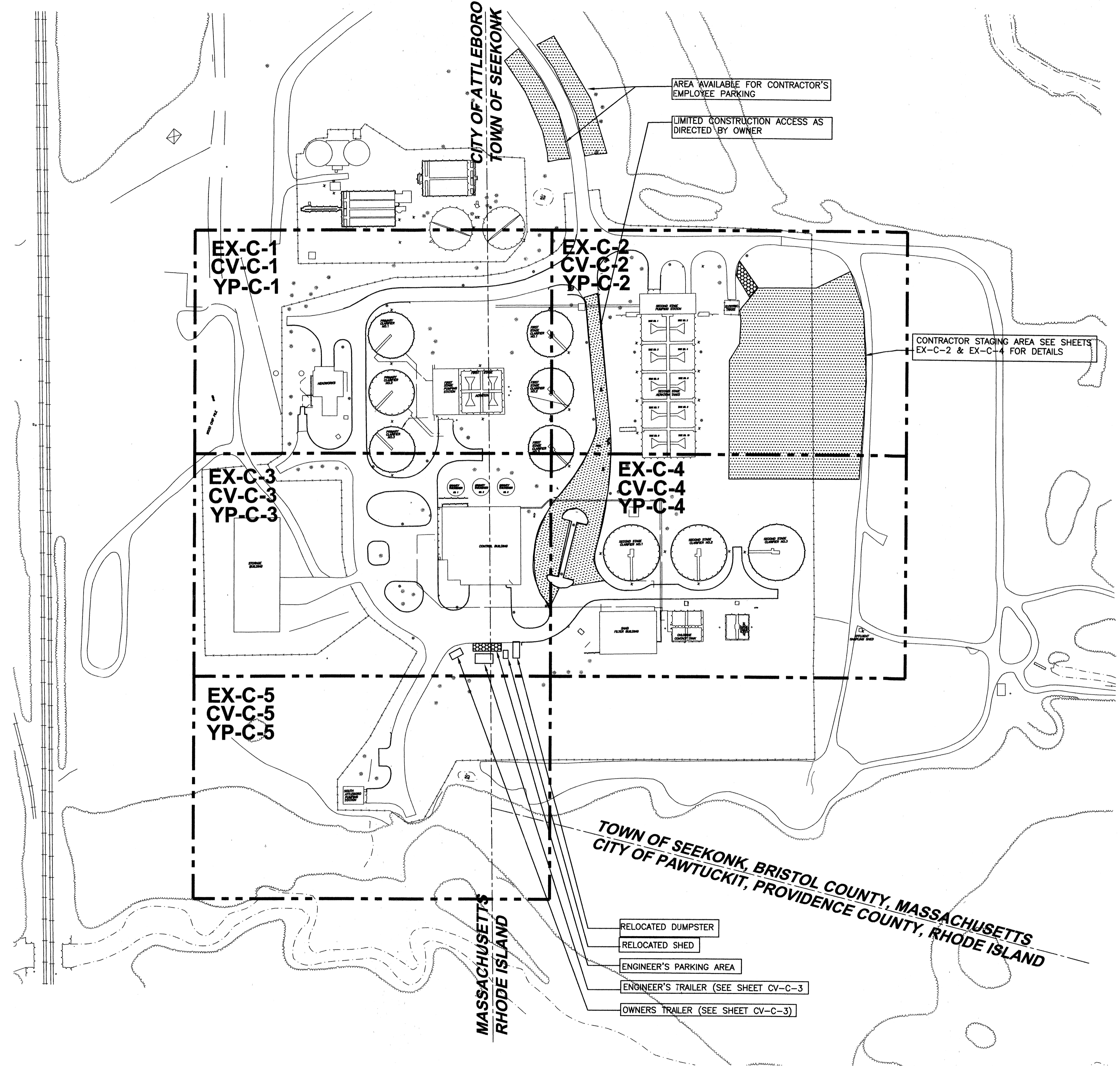
PLAN SCALE 1"=100'
