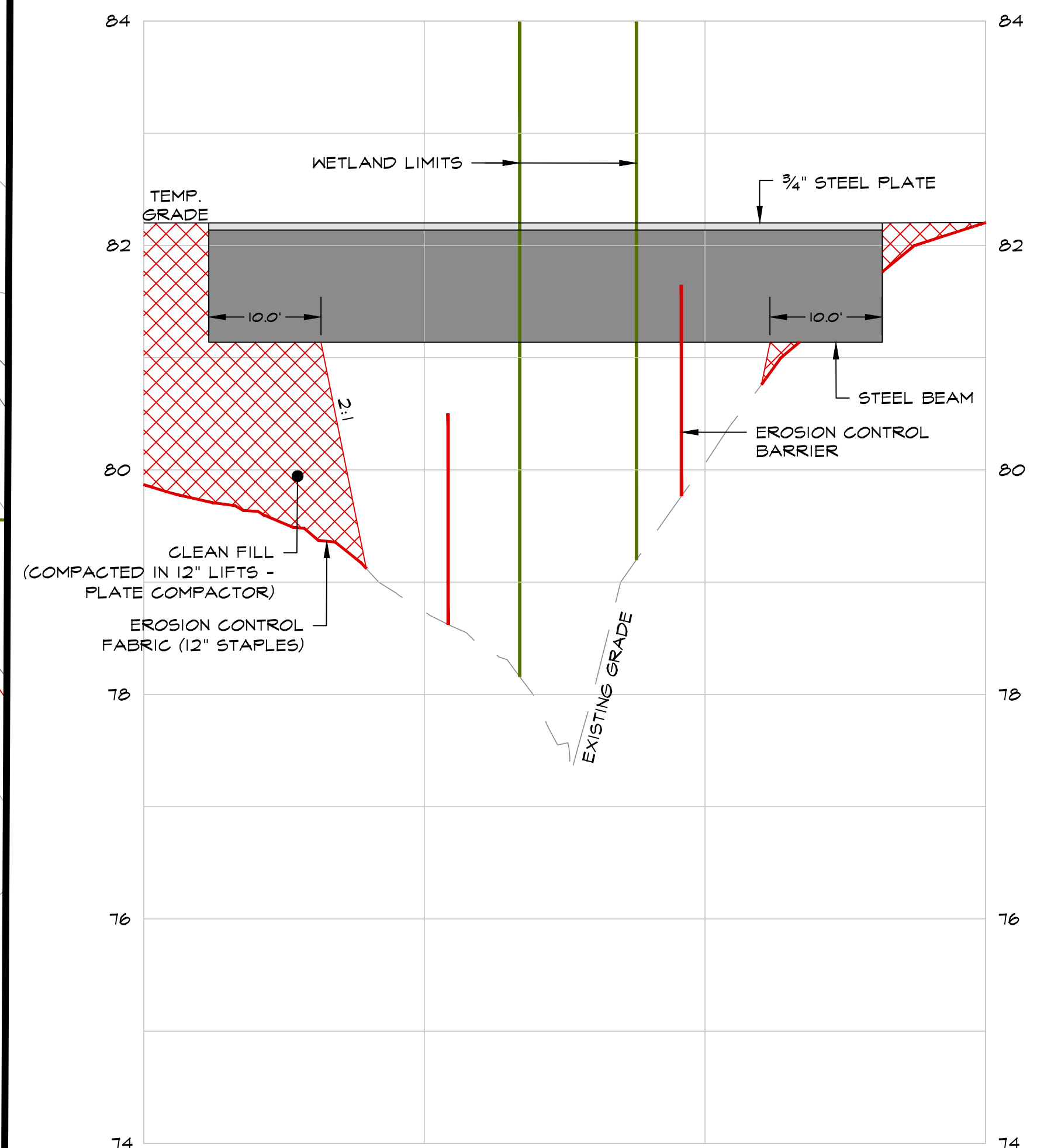
CROSS-SECTION B-B
