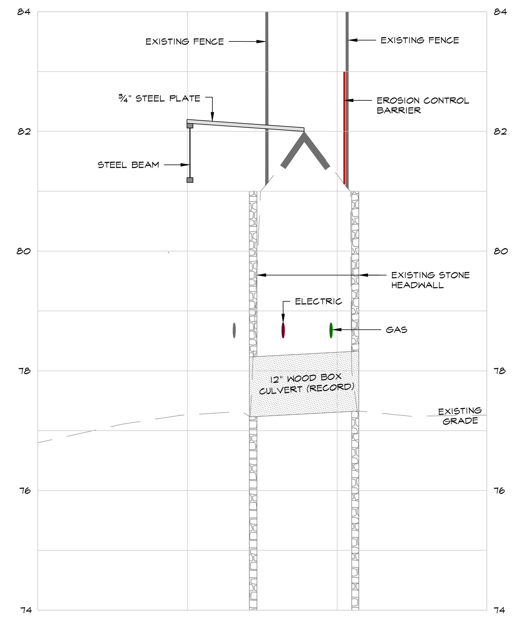
CROSS-SECTION A-A
